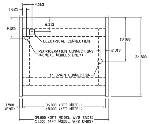
3' & 4' Plan Views
